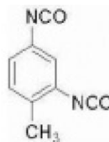
2,4-TDI
